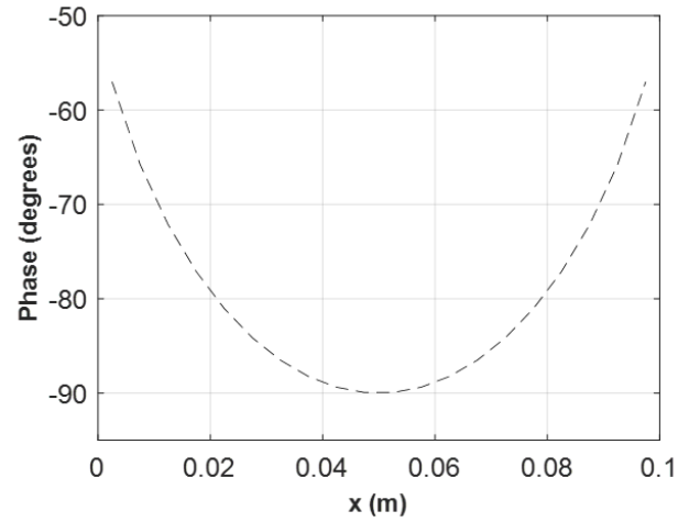
FIGURE 4. Phase angle phasor current density distribution over the bar width.
