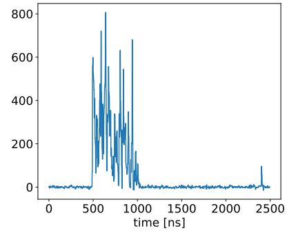
Figure 4. Scintillation in the THGEM recorded by the PMT.
