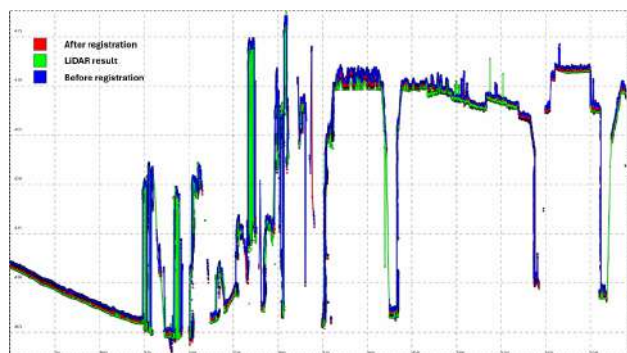
Figure 5. Vertical profile analysis demonstrating that the registered elevation (Red) aligns closely with the LiDAR reference (Green), significantly reducing the initial geometric drift (Blue).
