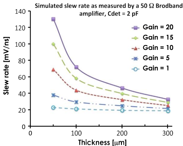
Fig. 7. Simulated UFSD slew rate as a function of gain and sensor thickness. Thin sensors with even moderate gain (10–20) achieve a much higher slew rate than traditional sensors (gain \approx 1).
