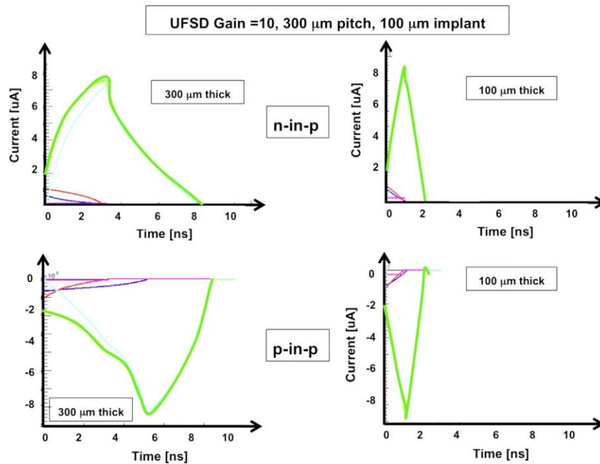
Fig. 10. Current signals in n-in-p and p-in-p UFSD sensors with gain/10, 300 μm pitch, and 100 μm implant. Left: thickness 1/4 300 μm, right: thickness 1/4 100 μm. The meaning of the various color is shown in Fig. 5. (For interpretation of the references to color in this figure caption, the reader is referred to the web version of this paper.)
