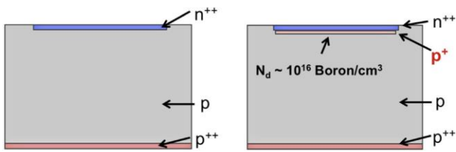
Traditional Silicon Diode Low Gain Avalanche Diode
