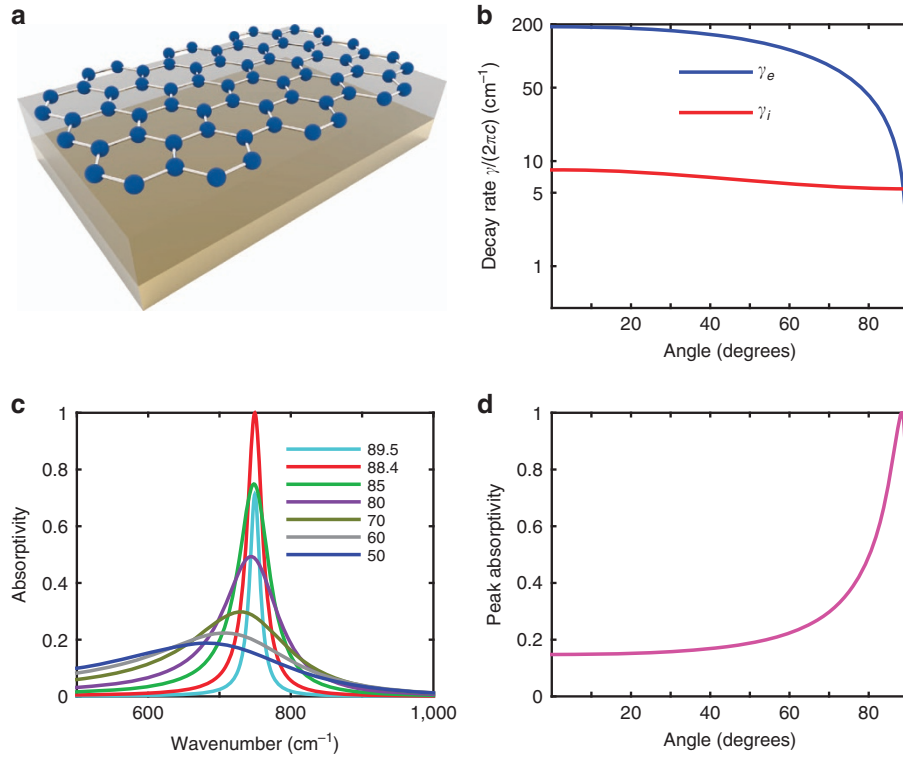
Figure 1 Decay rates and critical coupling. (a) Schematic of a structure consisting of a 2D material, separated from a mirror (light gray) by a dielectric spacer layer (dark gray). As an example, the 2D material is a single-layer graphene. (b) External and internal decay rates of the structure as a function of angle of incidence. The external decay rate ( \gamma_e , blue line) and internal decay rate ( \gamma_i , red line) are evaluated from Equations (7) and (8), respectively. (c) Calculated mid-infrared absorptivity of the structure, for varying angles of incidence. (d) Calculated peak absorptivity as a function of angle of incidence. In b , c and d , the structure consists of single-layer graphene separated from a PEC layer by a 1.9- \mu\text{m} -thick dielectric layer with a refractive index of 2.1. The graphene is assumed to have a Fermi energy of -500 meV with a mobility of 750 \text{ cm}^2 \text{ V}^{-1} \text{ s}^{-1} . In b , c and d , s-polarization is considered. PEC, perfect electric conductor.
