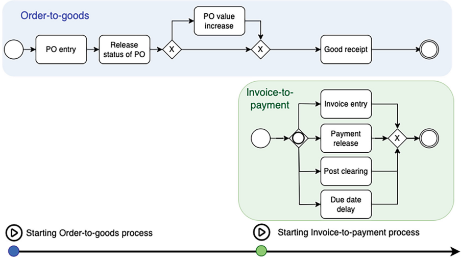
Fig. 3. Interaction between the Order-to-goods (PO) and Invoice-to-payment (IN) processes.
