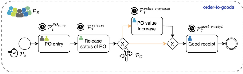
Fig. 1. Simulation model of order-to-goods process, composed of BPMN model ( \mathcal{N} ) and simulation parameters related to the resource ( \mathcal{P}_R ), time ( \mathcal{P}_T ), control flow ( \mathcal{P}_C ), and inter-arrival time ( \mathcal{P}_S ) perspectives.
