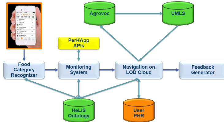
Fig. 1. Architecture of the end-to-end system. Green boxes are external resources, i.e., ontologies. Orange boxes are input data (pictures or PHRs). Light blue boxes are the modules of the system.
