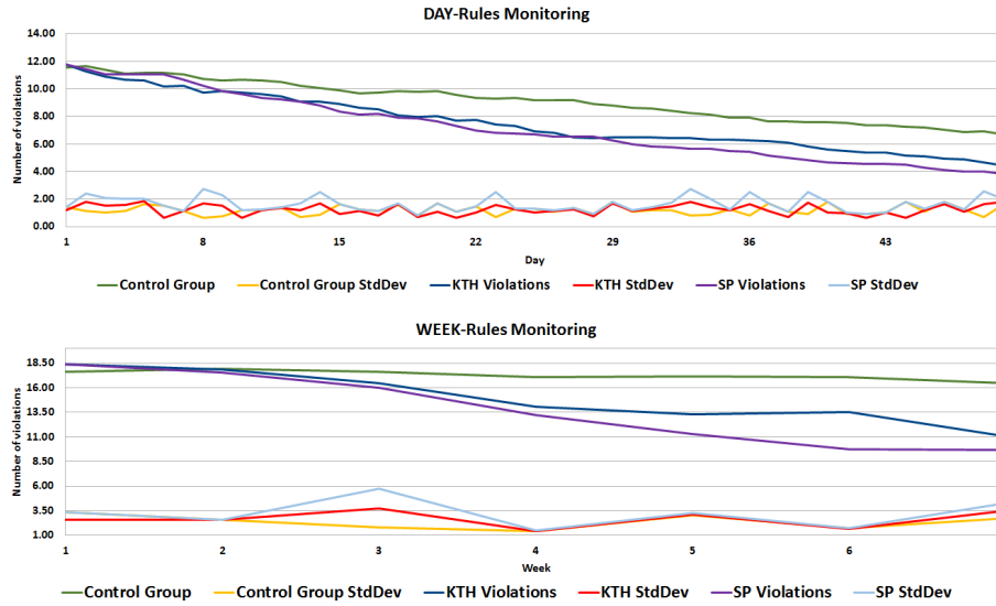
Fig. 3. Evolution of the average number of detected violations (per user), for the DAY and WEEK-Rules, during the Key To Health and Salute Plus observation period.
