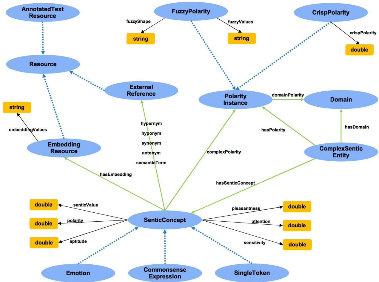
Figure 2: Overview of OntoSenticNet: each ellipse corresponds to one of the concepts composing OntoSenticNet; dashed arrows represents subsumption relationships; green arrows show the ObjectProperties; finally, black arrows describe the DatatypeProperties associated with each concept.
