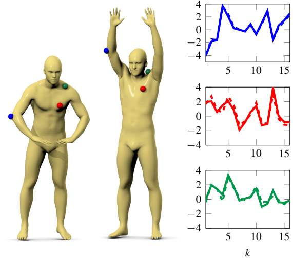
Figure 2: WFTs computed on two different poses of the same shape at three points marked in red, blue, and green. Solid lines represent the WFT of the shape on the left, dashed lines the ones of the shape on the right.
