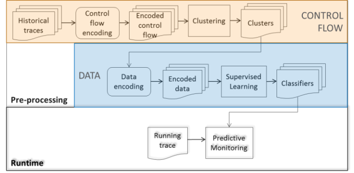
Fig. 4: PM Framework.
