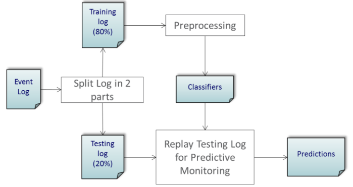
Fig. 5: Experimentation workflow.
