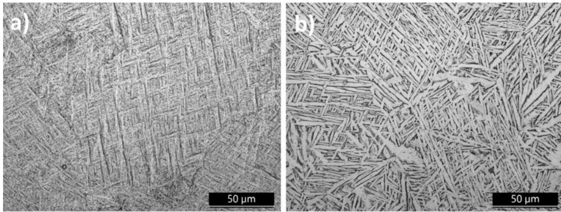
Fig. 4. Light optical micrographs of the microstructure of the Ti6Al4V ELI SLM sample in the as-received condition (a), after the HIP treatment (b).
