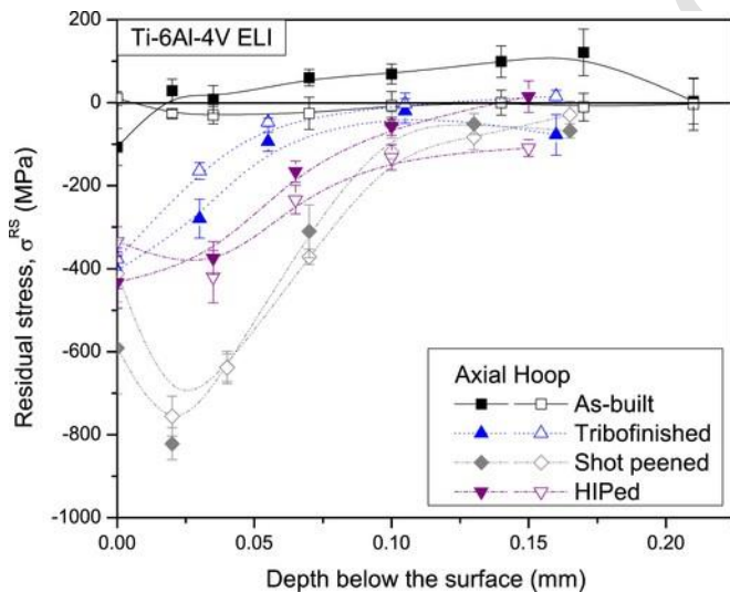
Fig. 8. Residual stress profiles measured by XRD technique.
