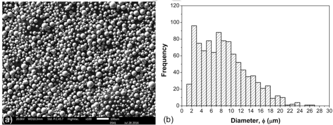
Fig. 1. (a) SEM micrograph of powder and (b) size distribution.
