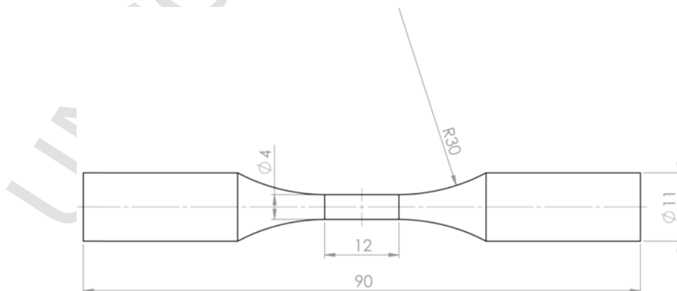
Fig. 2. Sample geometry used for push-pull fatigue tests (standard ASTM E606). Dimensions are in mm.
