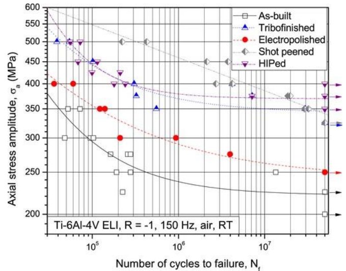
Fig. 9. Stress vs number of cycles to failure (S-N) curves of the investigated sample conditions.
