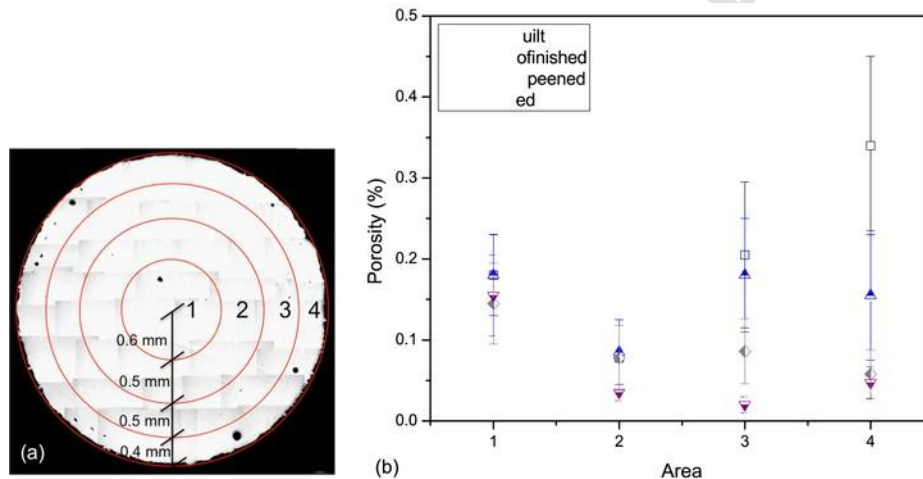
Fig. 5. Porosity of the samples. (a) Annular areas in which the cross-section is divided. The image is obtained by collating several optical micrographs (b) Results of the porosity measurements.
