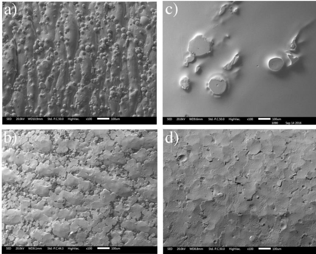
Fig. 6. SEM micrographs illustrating the surface morphology of the samples. (a) as-built, (b) tribofinished, (c) electropolished, (d) shot peened.
