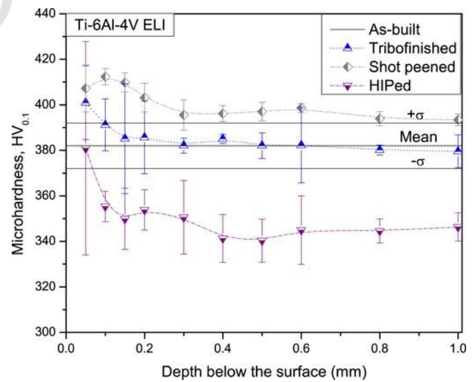
Fig. 7. Microhardness profiles, obtained by averaging the results of three tests.
