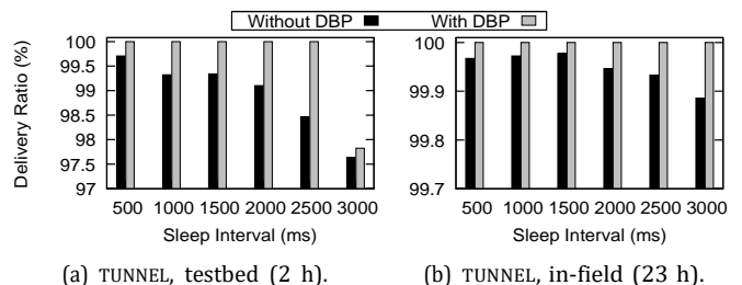
Fig. 11. Delivery ratio for the TUNNEL dataset.
