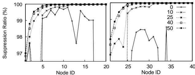
(b) Absolute error \epsilon^{abs} ( \epsilon^{rel} = 5\%, \epsilon_T = 0 ).
