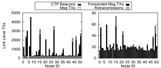
(a) INDOOR, testbed, without DBP. (b) INDOOR, testbed, with DBP.
