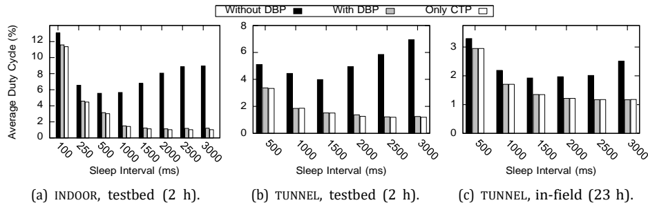
Fig. 12. Duty cycle. Note the varying y-axis scale.
