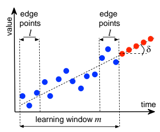
Fig. 2. Derivative-based Prediction.
