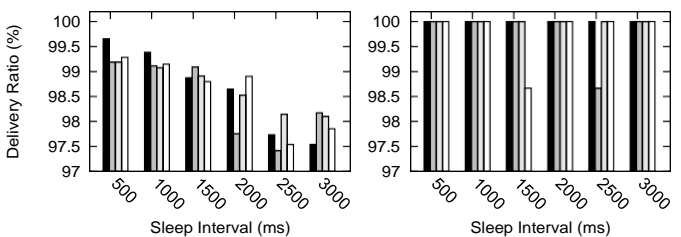
(c) Without DBP.
