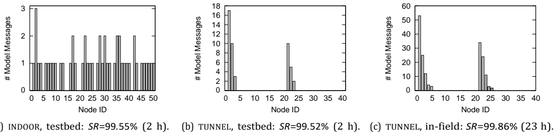
Fig. 10. Number of model update messages.
